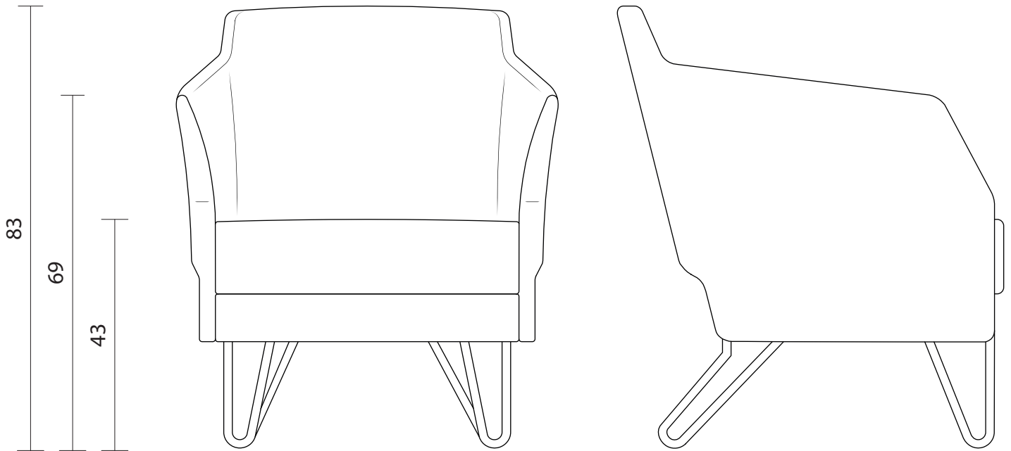
DAKOTA - Armchair shell with base (PL-DKT-000) (FB-DKT-100) + (SB-DKT-NE)
