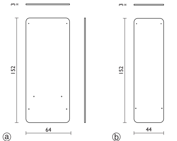
a: universal medium wall b: tight wall
