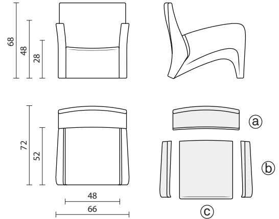
a: backrest b: left and right armrest c: seat
